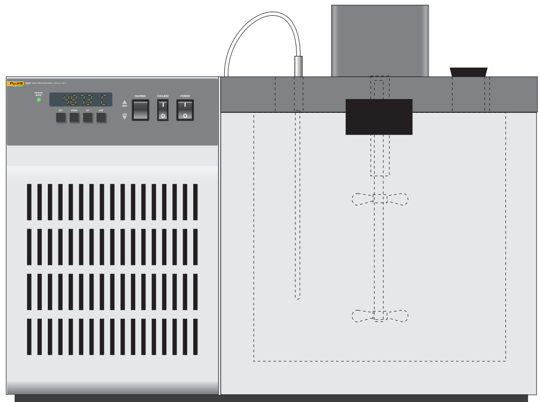
Figure 1 Bath Assembly
