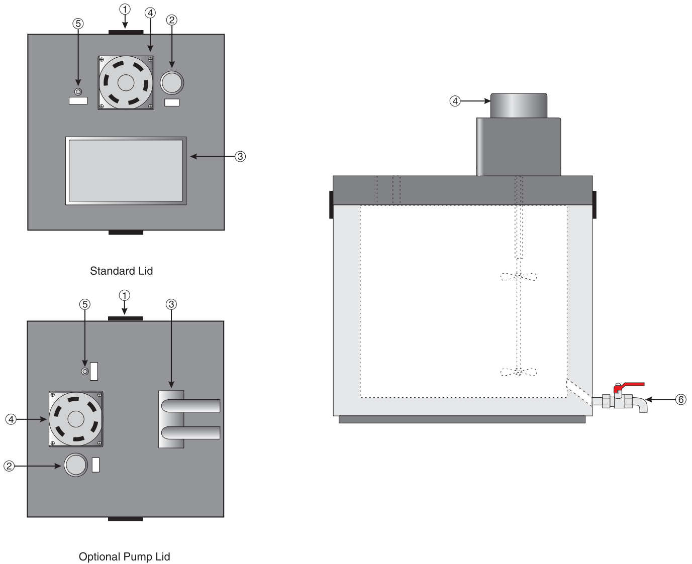
Figure 5 Drain Location and Lid Options
