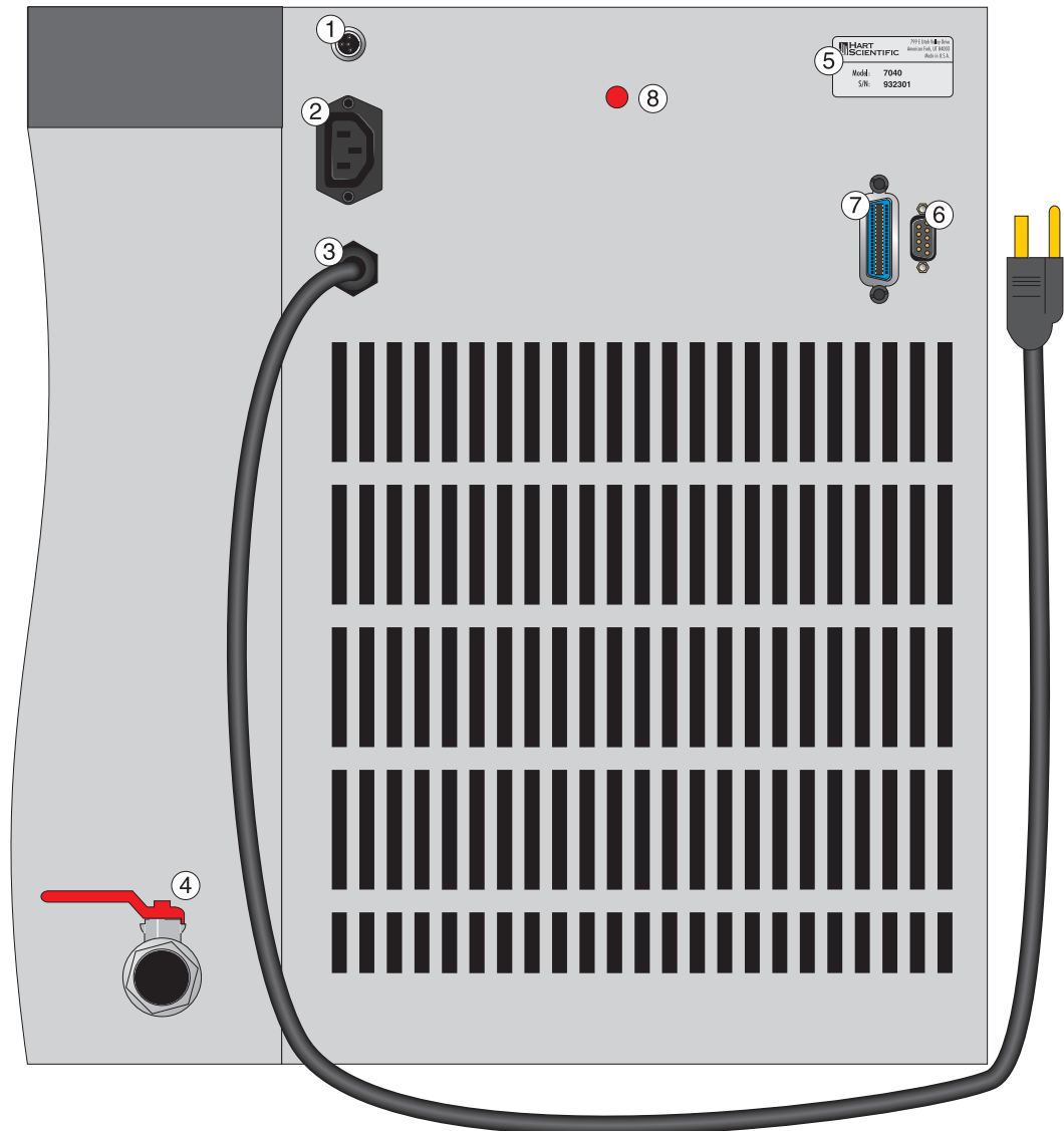
Figure 4 Back Panel
