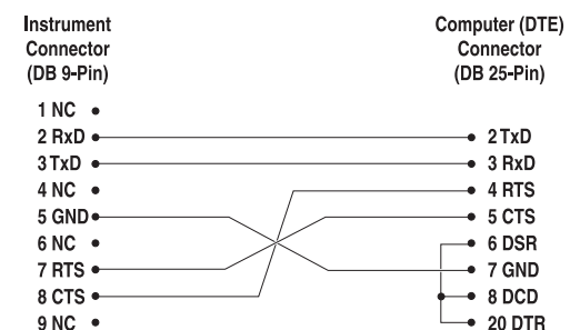
Figure 9 Serial Cable Wiring
